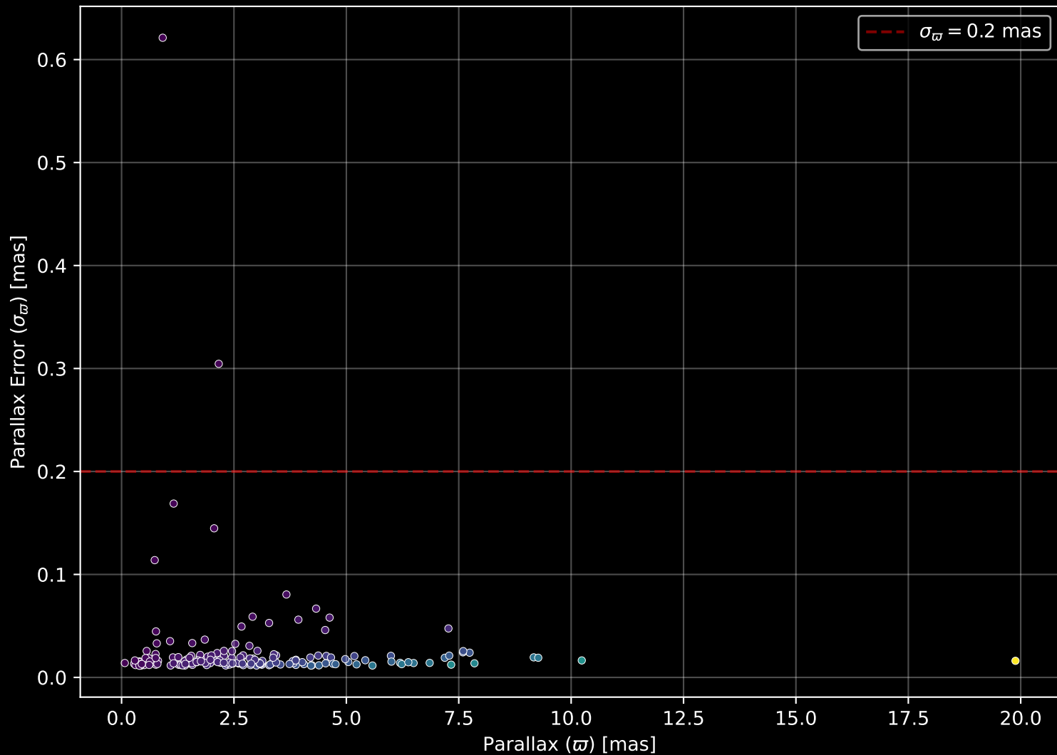
APOGEE DR17 Field: [JHelium3] Parallax Quality (n= 175)
