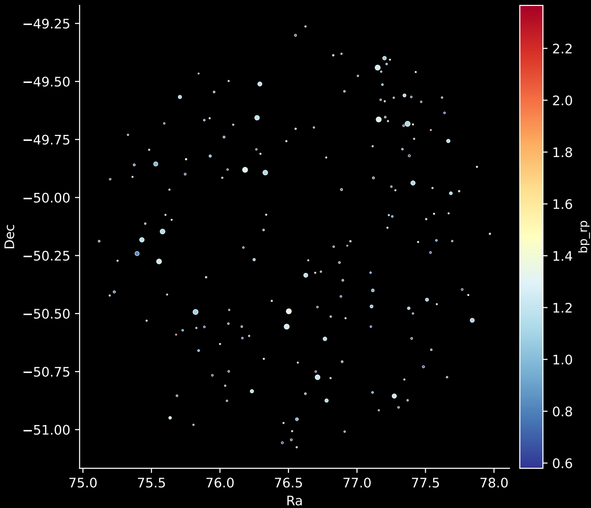
APOGEE DR17 Field: [JHelum3] Stars: 175
