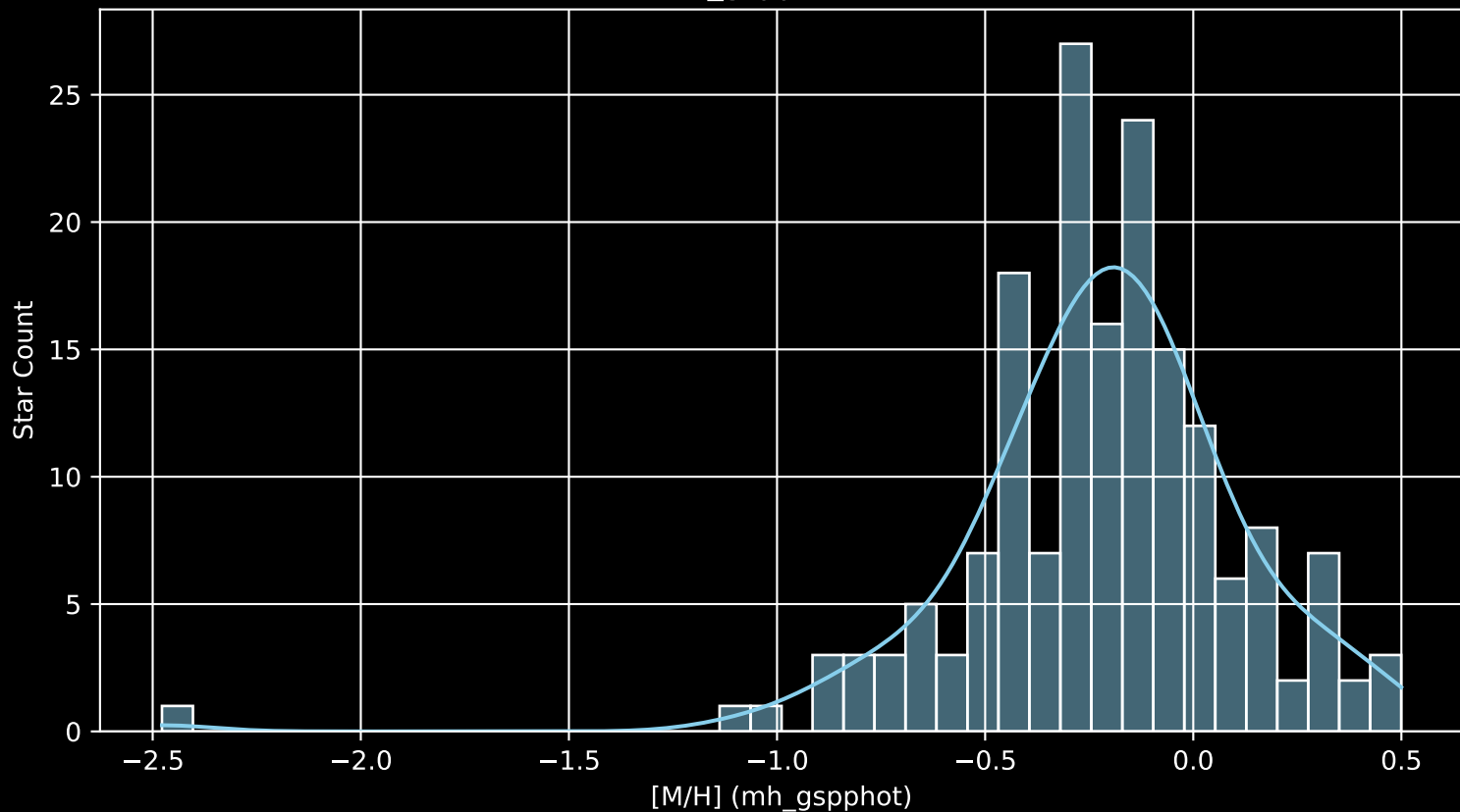
APOGEE DR17 Field: [JHelum3 [M/H] (mh_gspphot) (n= 174)
