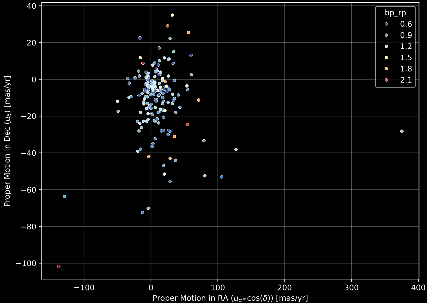
APOGEE DR17 Field: [JHelium3] Proper Motion Diagram (n= 175)
