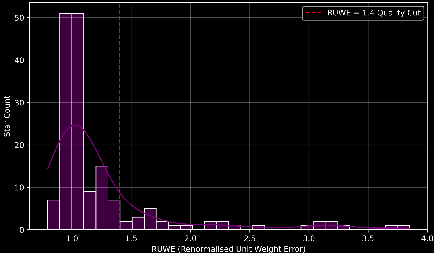
GAPOGEE DR17 Field [JHelium3] RUWE Distribution (n= 168)
