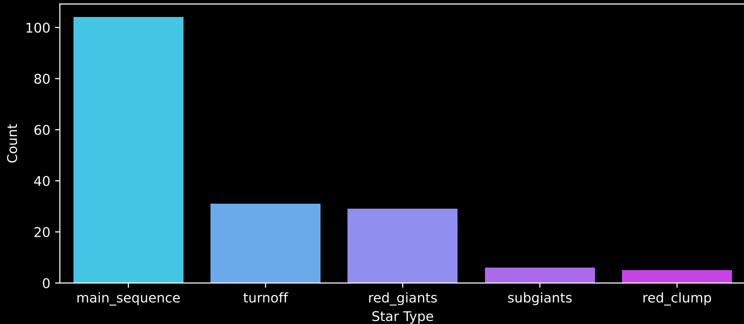
APOGEE DR17 Field: [JHelum3] Count plot of Star Type
