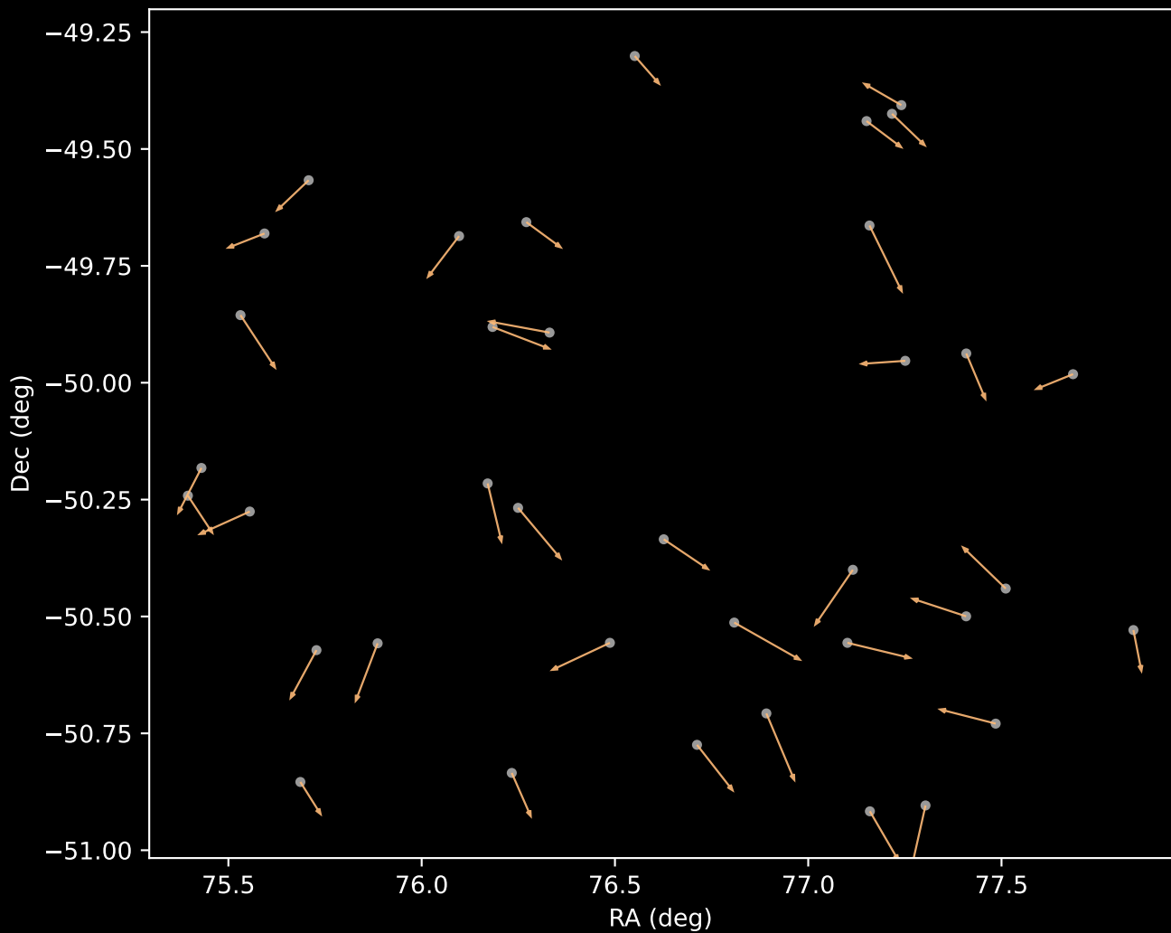
APOGEE DR17 Cluster 3 Proper Motion Vectors (n=37)
